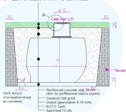
INSTALLATION BELOW TRAFFIC SURFACES
