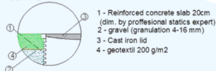
DETAIL A
